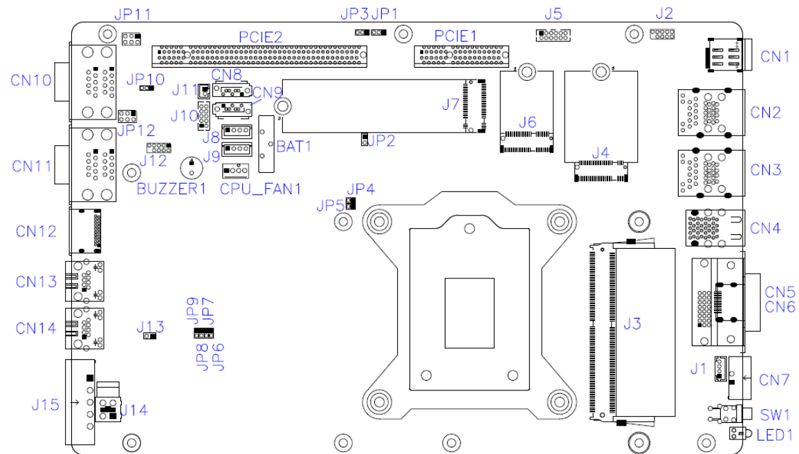
MB230 Motherboard
