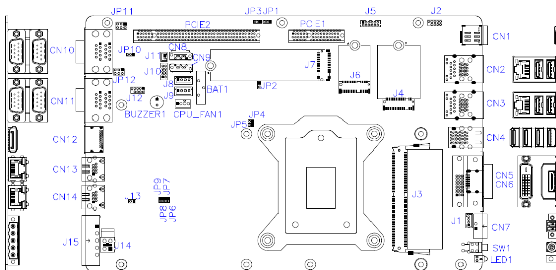
MB230 Motherboard
