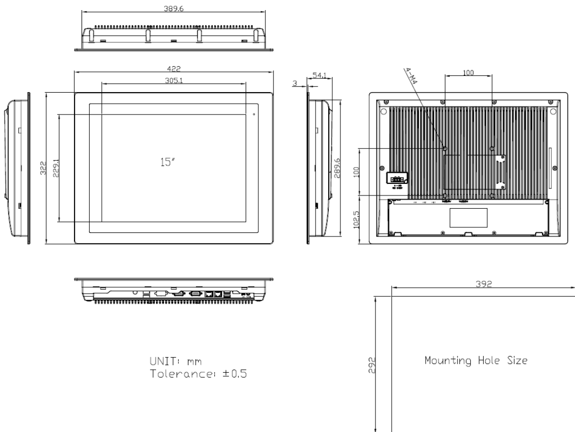
Figure 1.4: Dimensions of FABS-815P/G(H)
