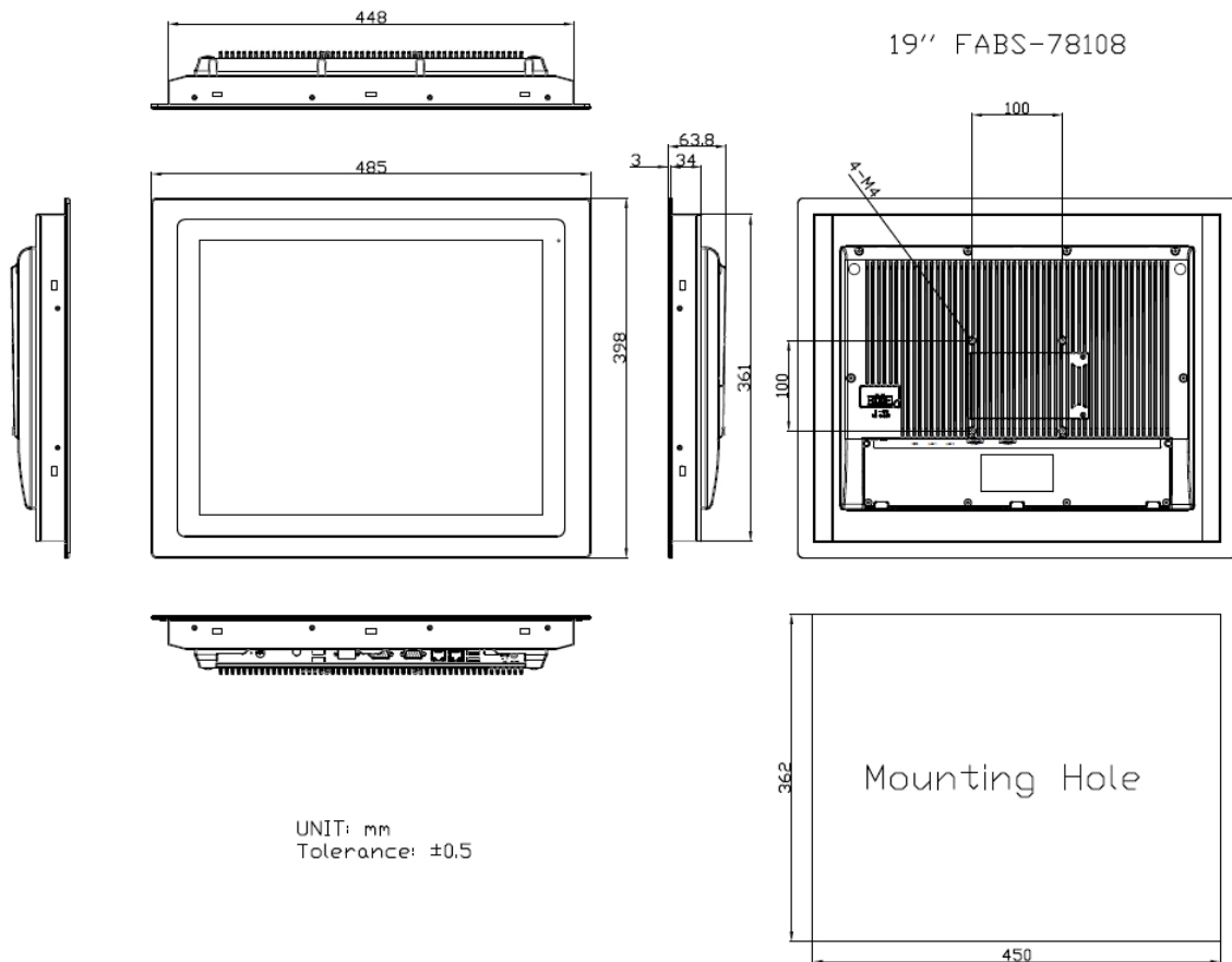
Figure 1.6: Dimensions of FABS-819P/G(H)
