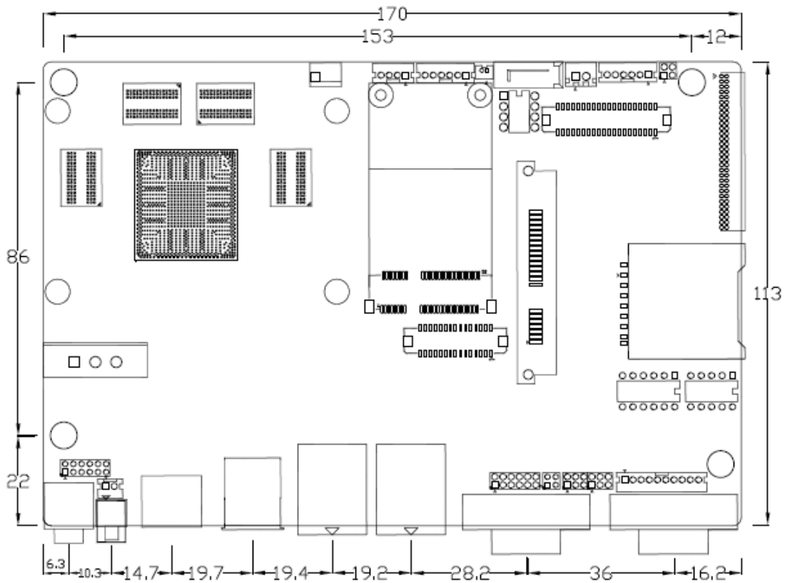
Figure 2.1: Motherboard Dimensions
