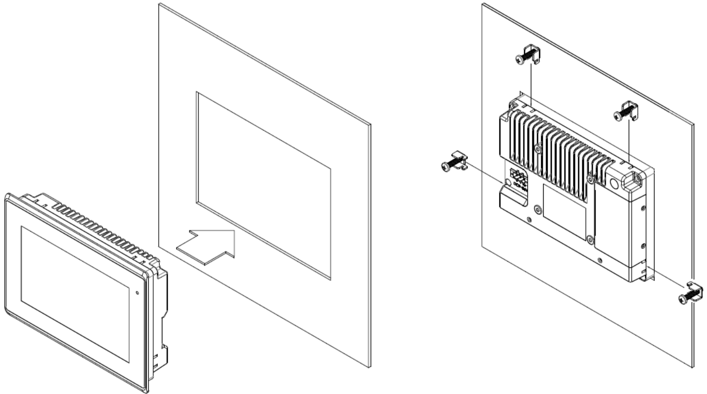
Figure 1.10: Panel Mounting of FABS Series
