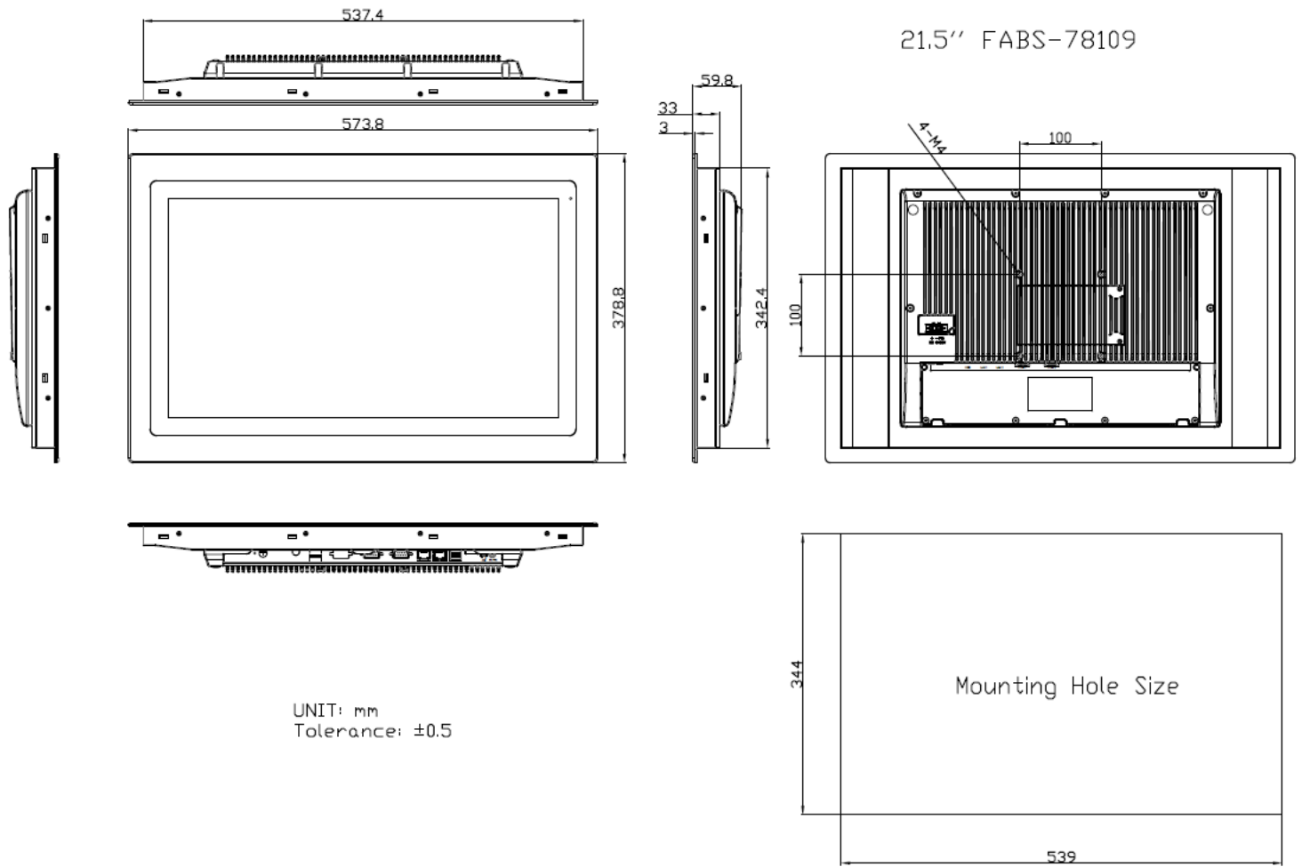
Figure 1.7: Dimensions of FABS-821P/G(H)9
