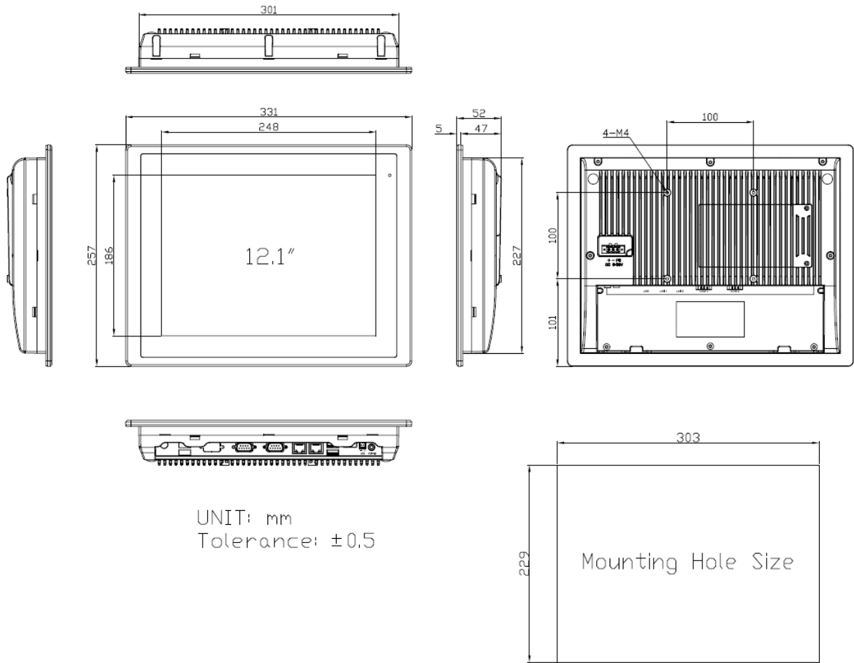
Figure 1.3: Dimensions of FABS-812P/G(H)
