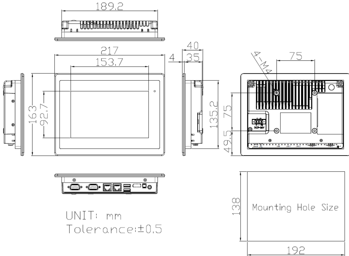
Figure 1.1: Dimensions of FABS-807P/G(H)
