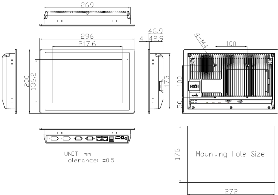
Figure 1.2: Dimensions of FABS-810P/G(H)
