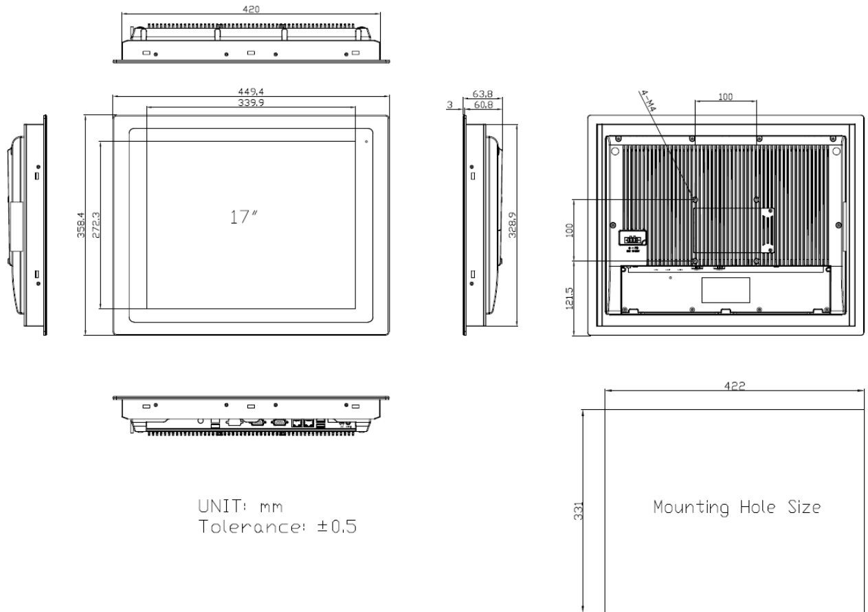
Figure 1.5: Dimensions of FABS-817P/G(H)
